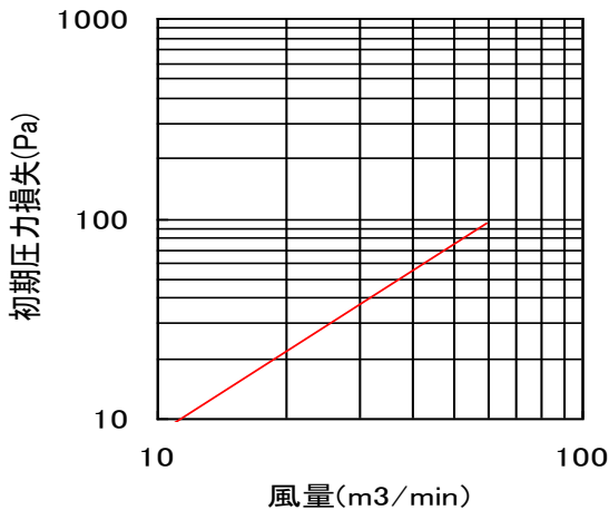
捕集効率 65%
